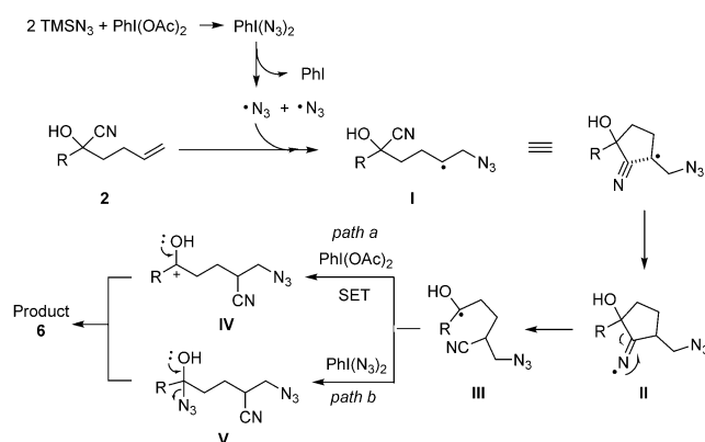
Figure 1. Proposed mechanism.
